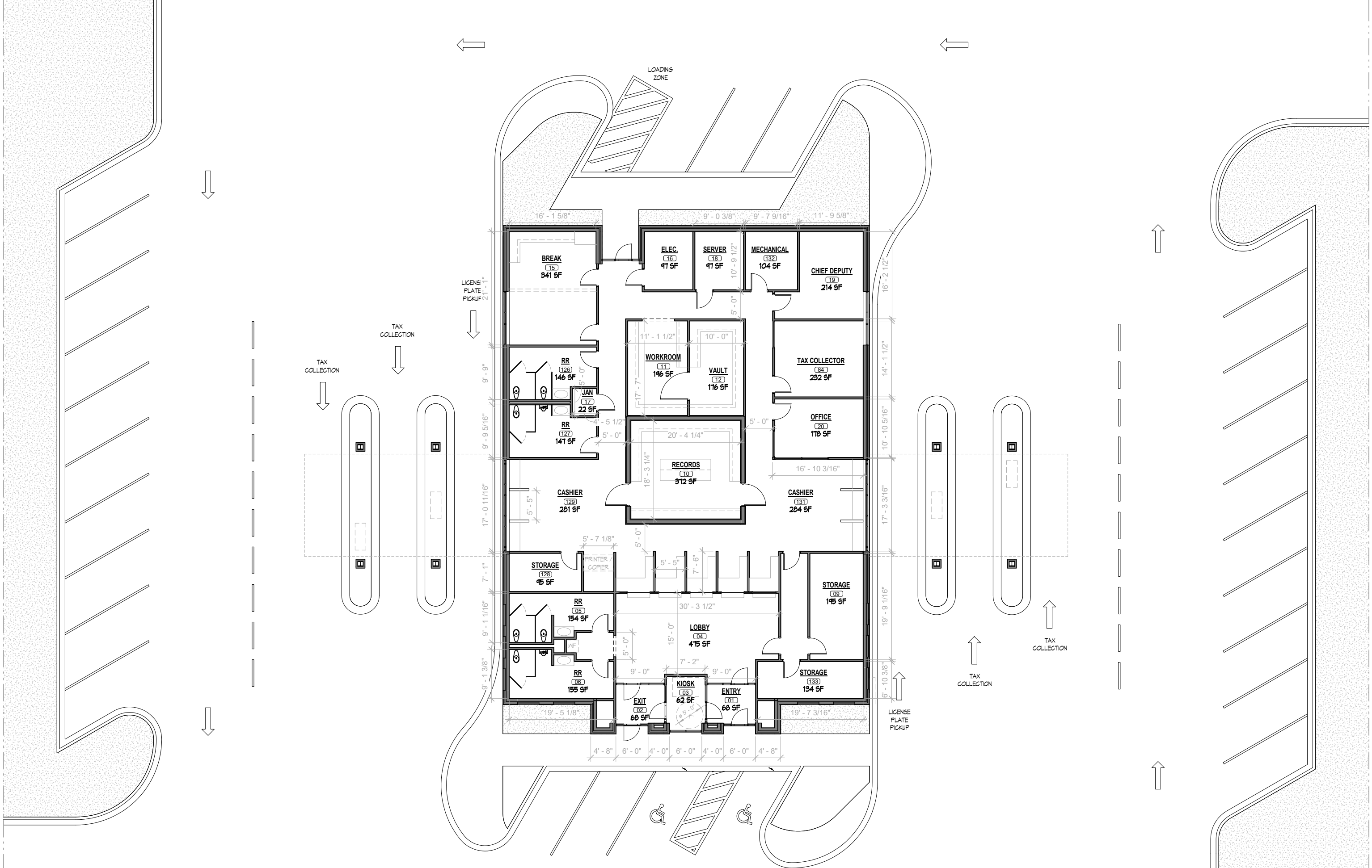
FLOOR PLAN V26 SC: 1/16" = 1' - 0" 6,200 GSF
