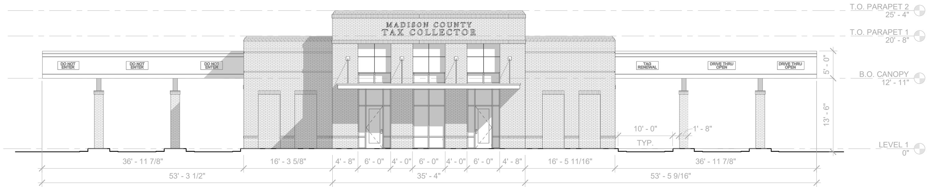
FRONT ELEVATION v11 SC: 3/32" = 1' - 0"
